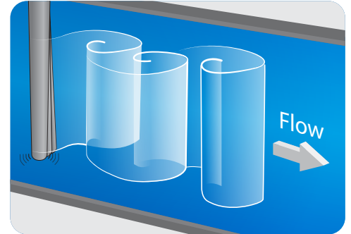
Standard Thermowell
